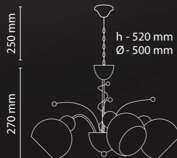
Lime 05 146 10M-3 3×E14×60W 390×303×325 (0.039 m³)
